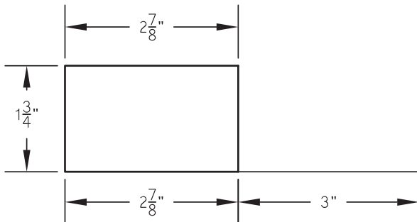
QuickLiner TS Curb Cover - Front View
