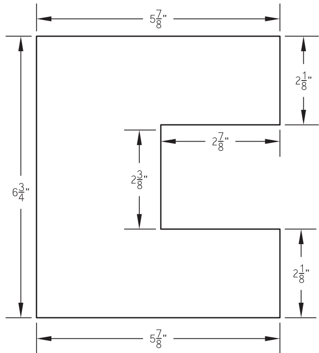
QuickLiner TS Curb Cover - Top View
